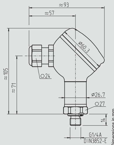
with field case
