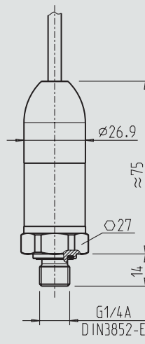
with cable outlet IP 68, FEP, IP 6K9K
